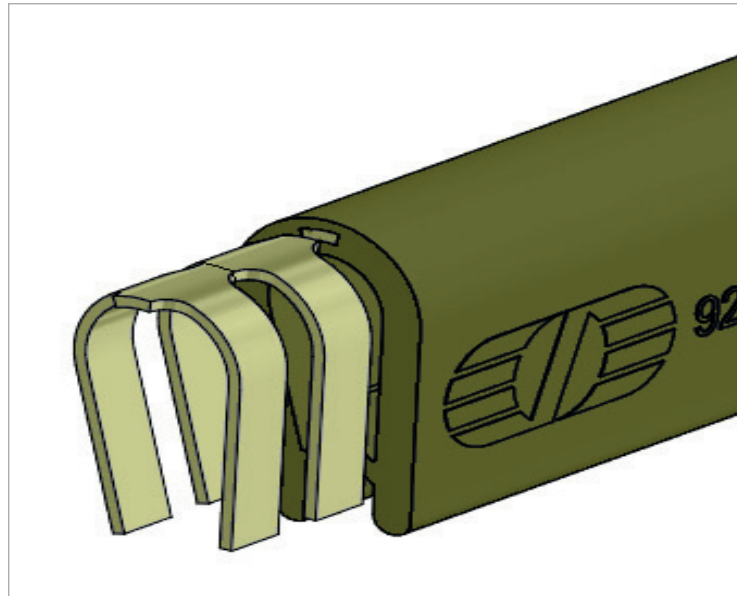
Individual SS legs are encapsulated in EPDM rubber
